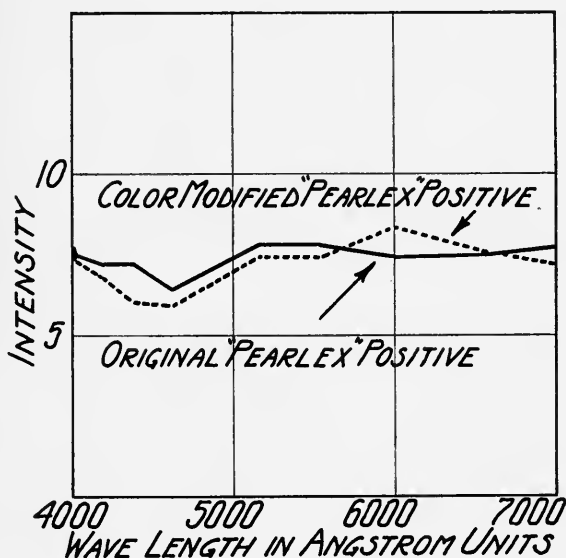
FIG. 1. Spectral energy distribution of positive crater radiation from 6-mm "National" "Pearlex" Positive—5.5-mm "National" "Pearlex" Negative at 30 amperes, 28 volts d-c.
